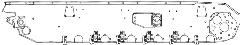
Above and Below: A partially completed Pz.Kpfw.III Ausf.F Fahrgestell with the bases for the final drive, shock absorbers and track tensioner installed, as well as the Schwingarmfuehrung (guides for the swing arms).
