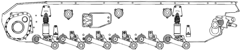
Above and Below: A partially completed Pz.Kpfw.III Ausf.F Fahrgestell with the final drive, return rollers, shock absorbers, track tensioner, bump stops, and swing arms installed.
