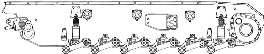
Above and Below: A partially completed Pz.Kpfw.III Ausf.F Fahrgestell with the final drive, return rollers, shock absorbers, track tensioner, bump stops, and swing arms installed.
