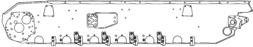
Above and Below: A partially completed Pz.Kpfw.III Ausf.F Fahrgestell with the bases for the final drive, shock absorbers and track tensioner installed, as well as the Schwingarmfuehrung (guides for the swing arms).
