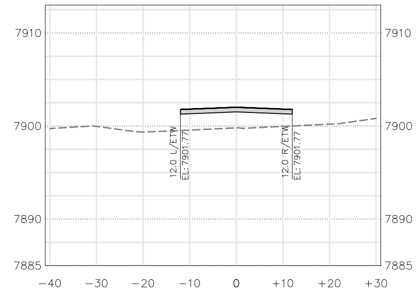
PUBLIC ROAD-1 (72+00)
