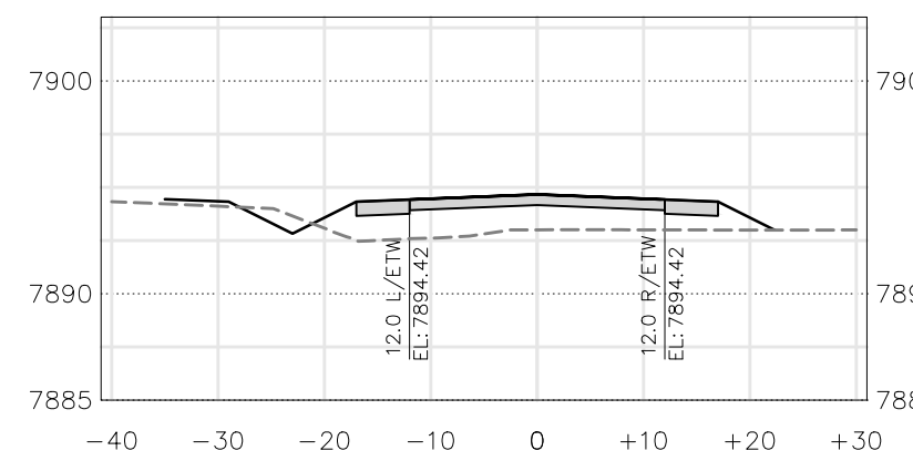
PUBLIC ROAD-1 (66+00)
