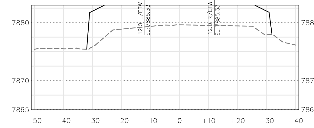
PUBLIC ROAD-1 (31+50)
