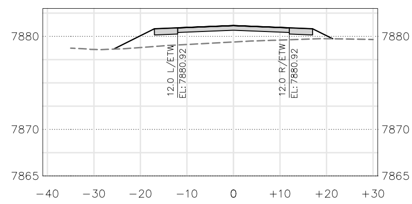
PUBLIC ROAD-1 (40+00)
