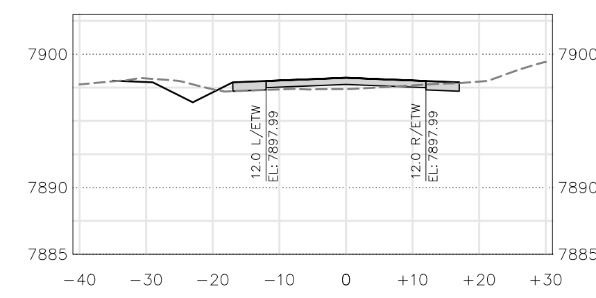
PUBLIC ROAD-1 (75+00)
