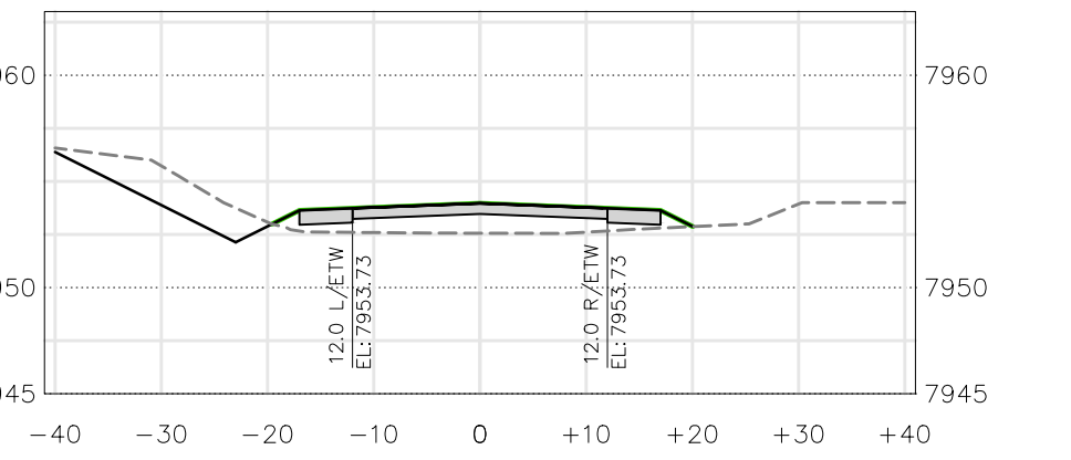
PUBLIC ROAD-1 (135+50)
