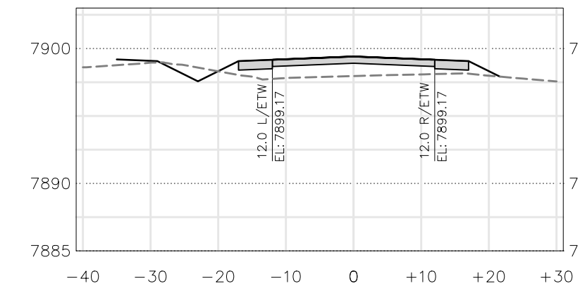
PUBLIC ROAD-1 (67+50)
