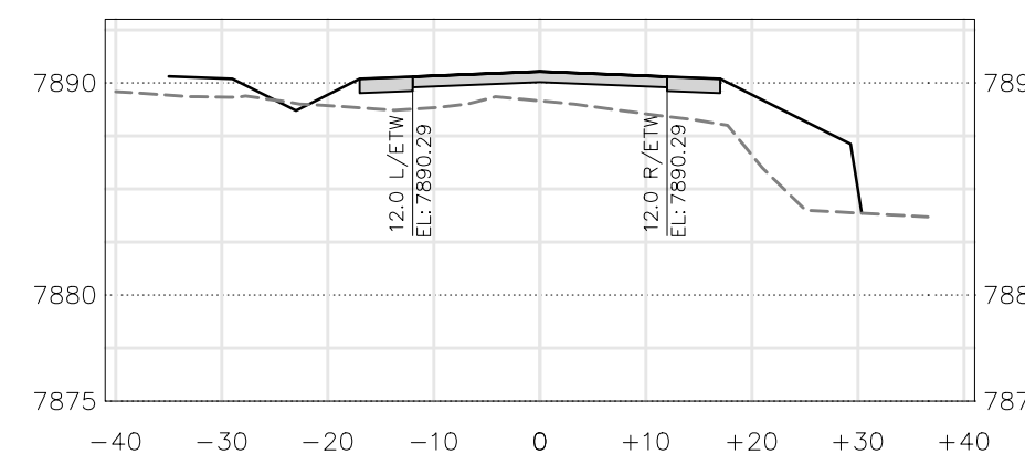
PUBLIC ROAD-1 (79+00)
