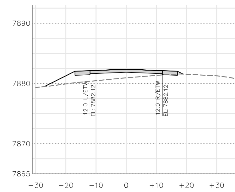
PUBLIC ROAD-1 (26+50)
