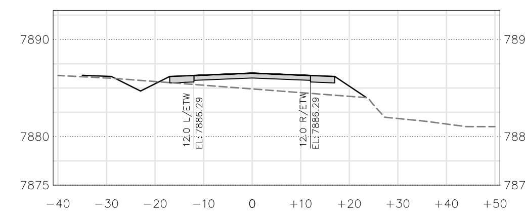
PUBLIC ROAD-1 (80+00)
