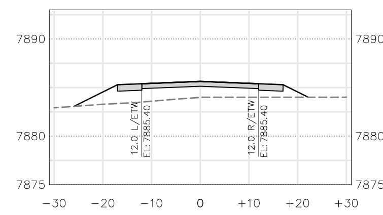
PUBLIC ROAD-1 (54+50)
