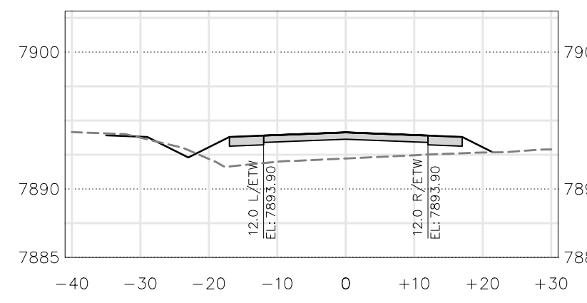
PUBLIC ROAD-1 (65+50)
