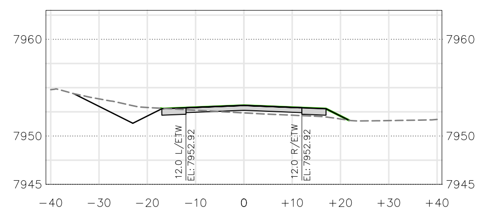
PUBLIC ROAD-1 (130+00)
