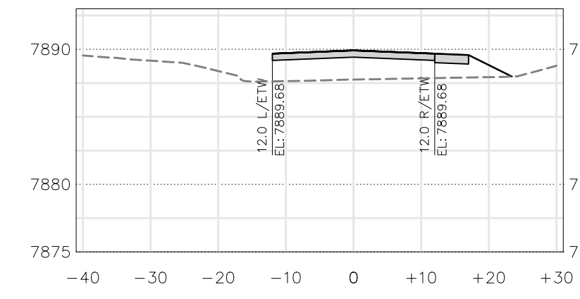
PUBLIC ROAD-1 (58+50)
