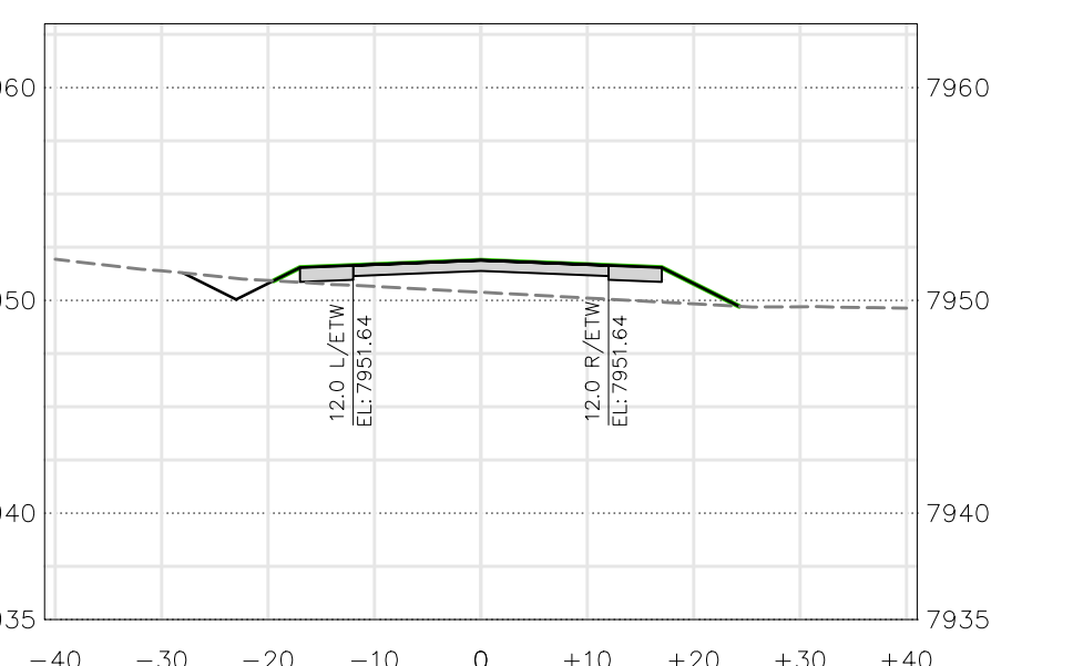
PUBLIC ROAD-1 (128+00)
