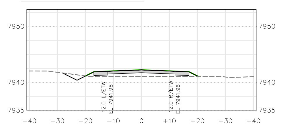
PUBLIC ROAD-1 (122+50)
