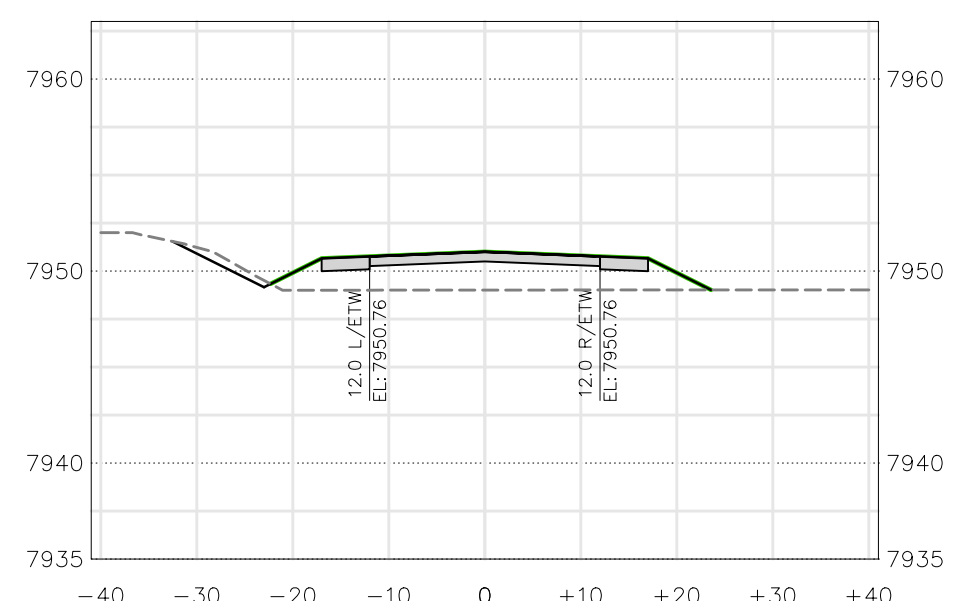
PUBLIC ROAD-1 (127+50)
