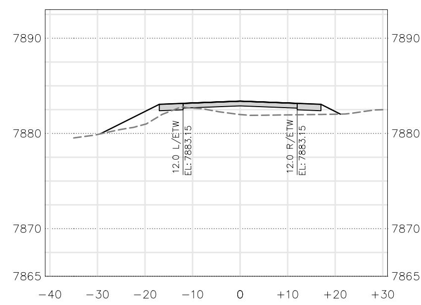
PUBLIC ROAD-1 (38+50)
