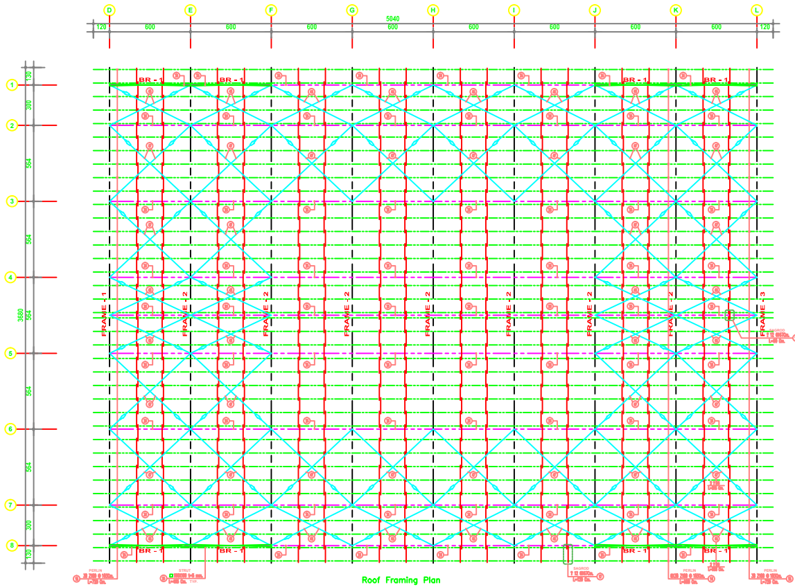
Roof Framing Plan SC 1/100
