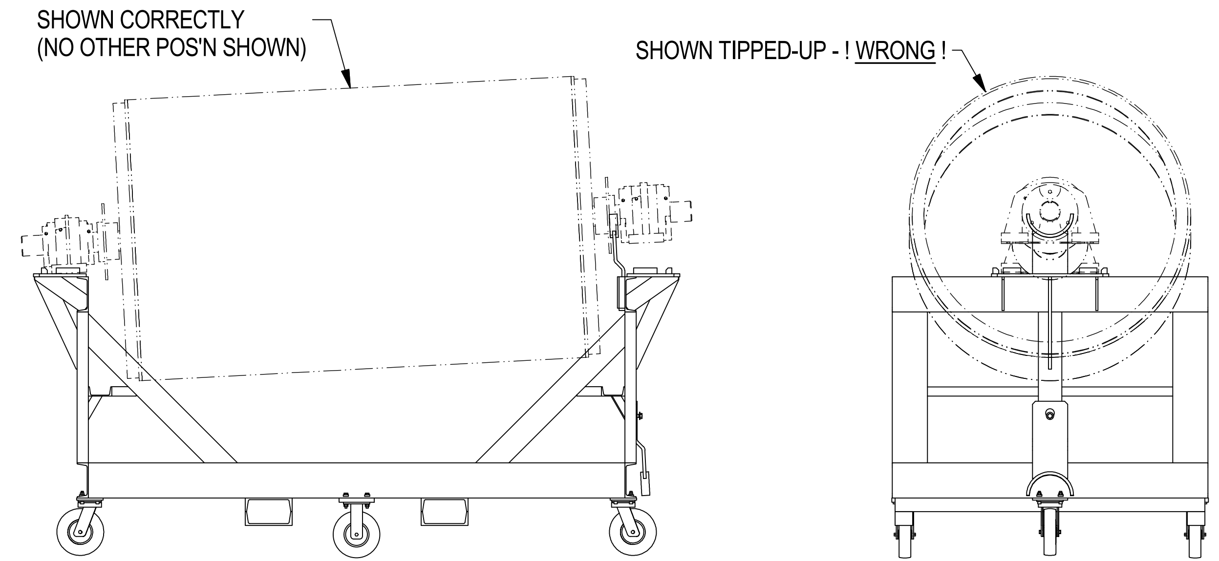
DRAWING VIEW-POSITION SCALE 1:16
