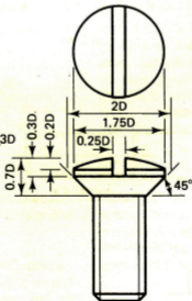
(e) Instrument or raised countersunk head
