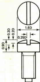
(f) Fillister head
