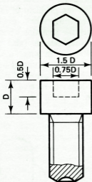
(g) Socket head
