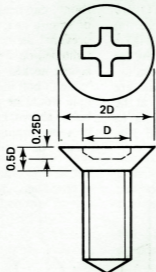
(h) Recessed head (countersunk screw)
