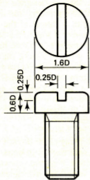
(a) Cheese head
