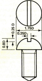
(c) Round head
