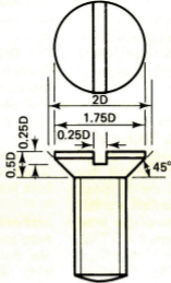
(b) Countersunk head
