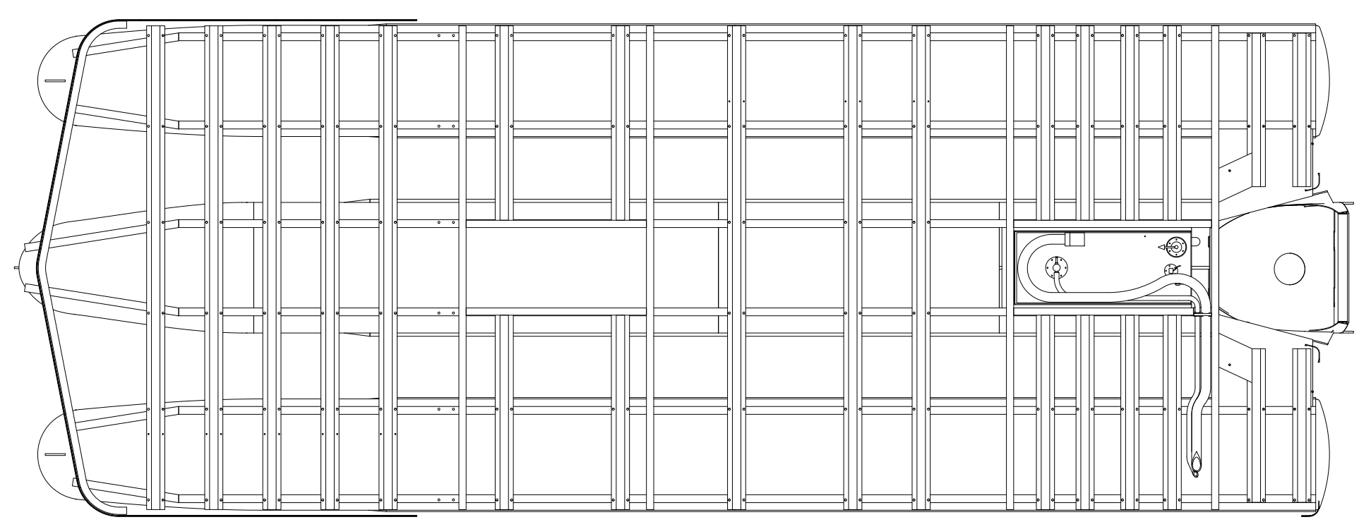
SECTION F-F SCALE 1/28
