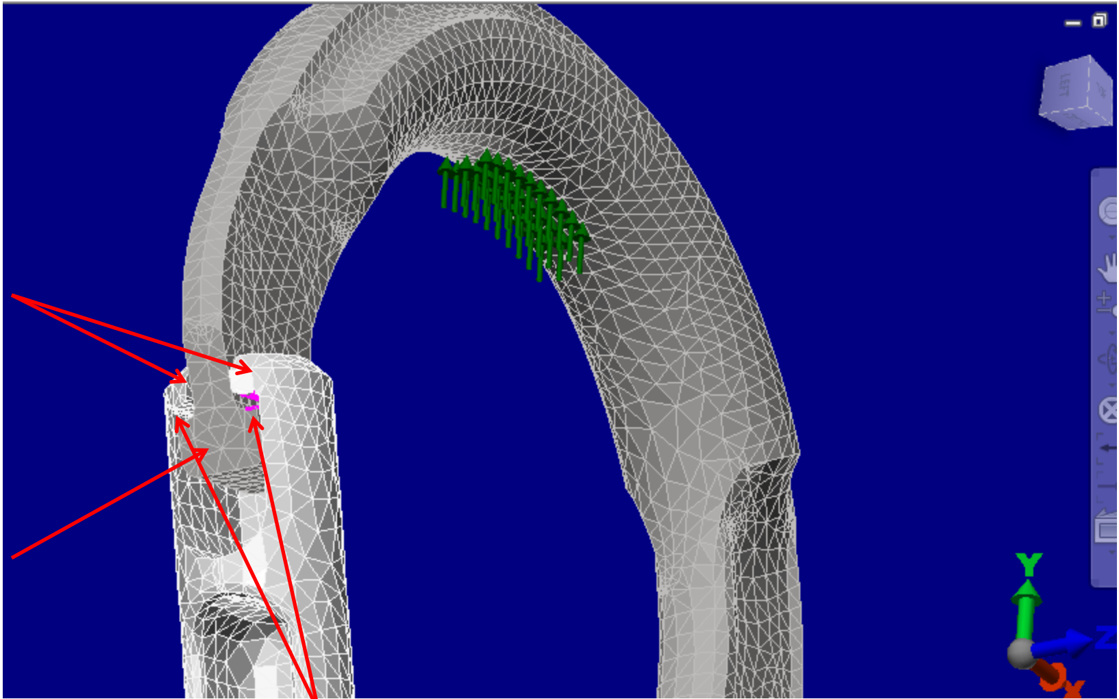
Contact regions with starting gap of 0.040"
