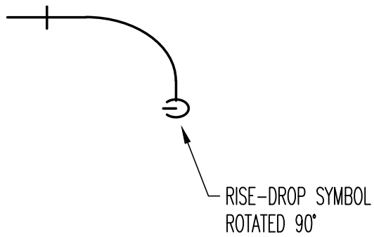
CONDUIT ELBOW ROTATED 45° DOWN RISE-DROP DISPLAYED INCORRECTLY
