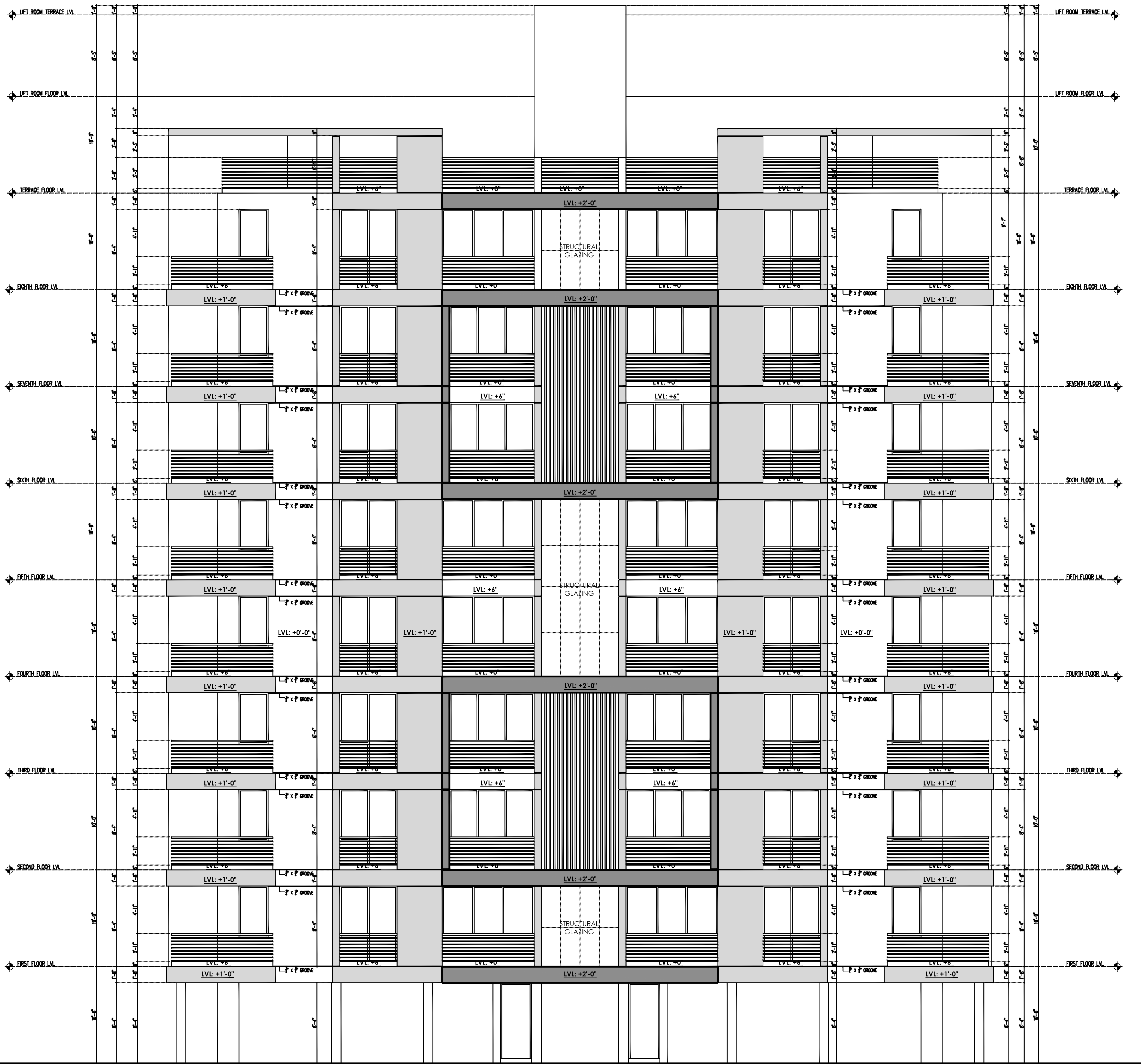
EAST SIDE ELEVATION(TOWER D)
