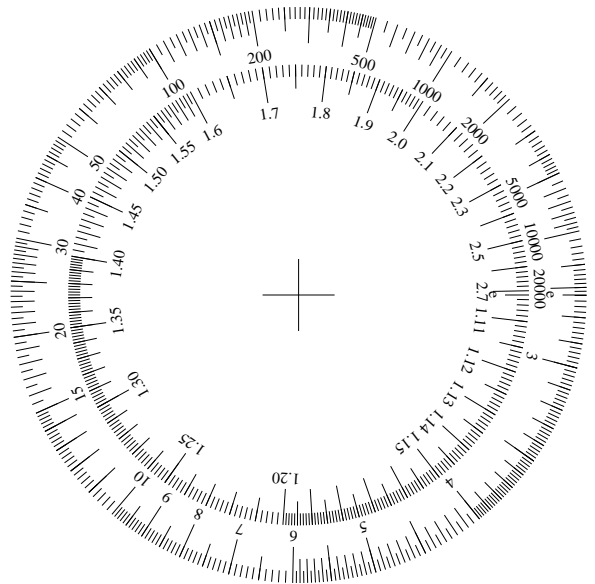
SIDE 2: OUTER SCALE
