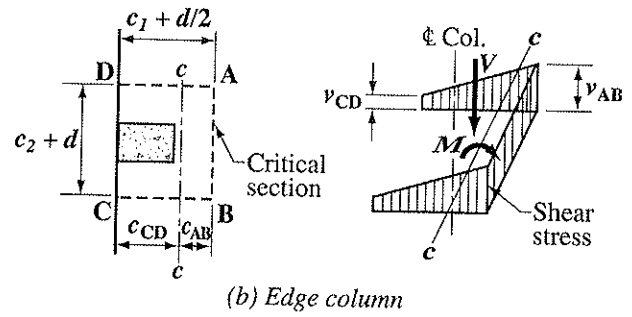
Fig. R11.12.6.2—Assumed distribution of shear stress
