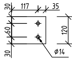
pl 42 Plate 8x120 Top view scale 1:10
