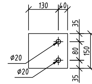
pl 49 Plate 10x150 Top view scale 1:10
