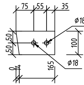
pl 47 Plate 10x100 Top view scale 1:10
