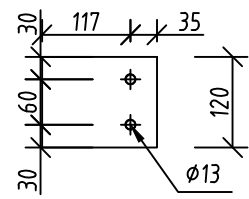
pl 43 Plate 8x120 Top view scale 1:10
