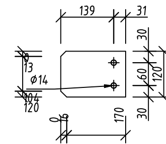
pl 48 Plate 8x120 Top view scale 1:10
