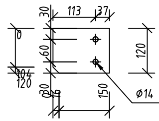
pl 41 Plate 8x120 Top view scale 1:10
