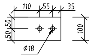
pl 50 Plate 10x100 Top view scale 1:10
