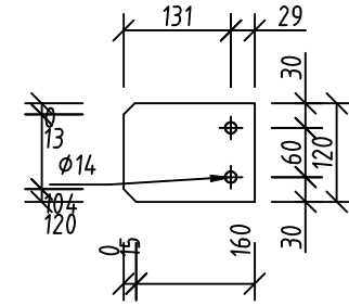
pl 44 Plate 8x120 Top view scale 1:10
