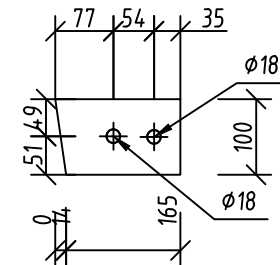
pl 46 Plate 10x100 Top view scale 1:10
