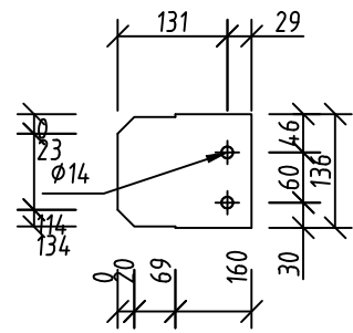
pl 45 Plate 8x136 Top view scale 1:10
