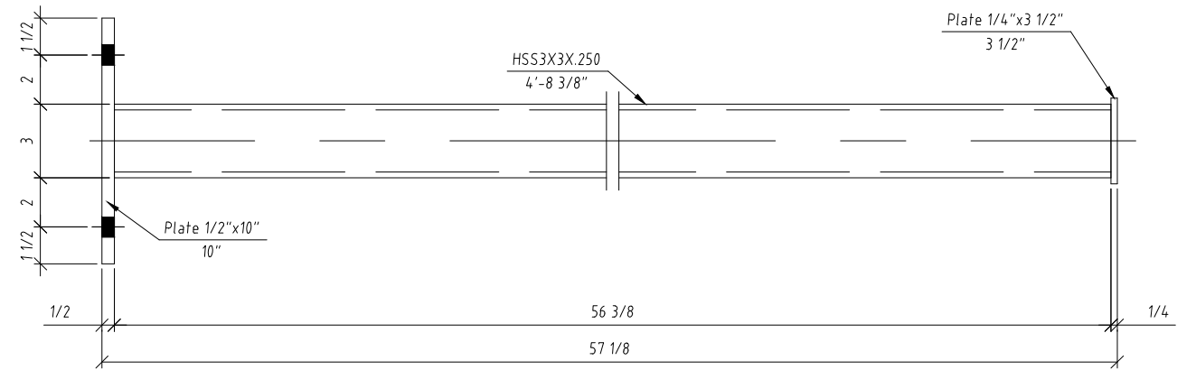
EXPLODED AND EDITED (STRETCHED) DRAWING
