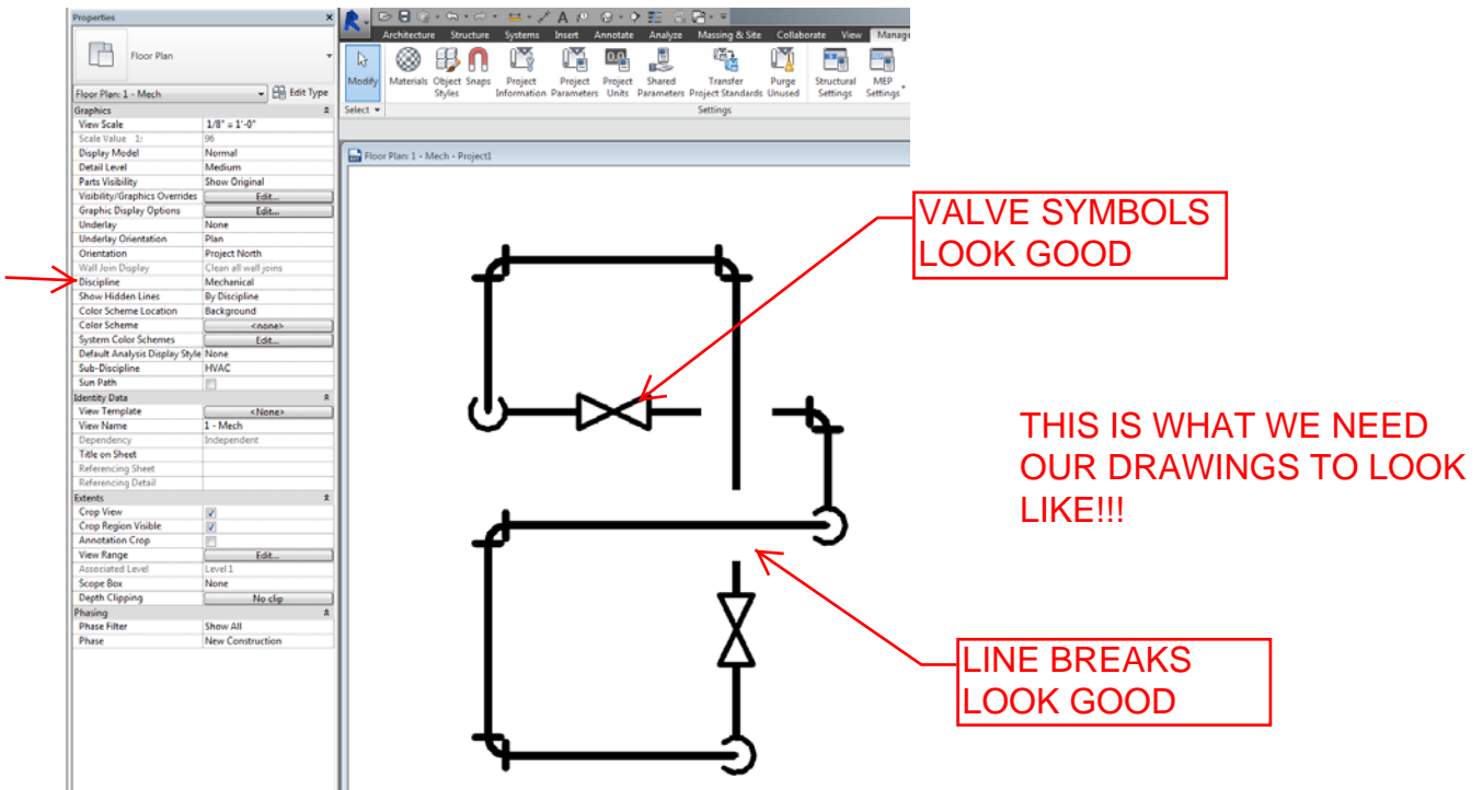
Figure 2 – SCREEN SHOT - PLAN VIEW IN REVIT (MECH DISCIPLINE)
