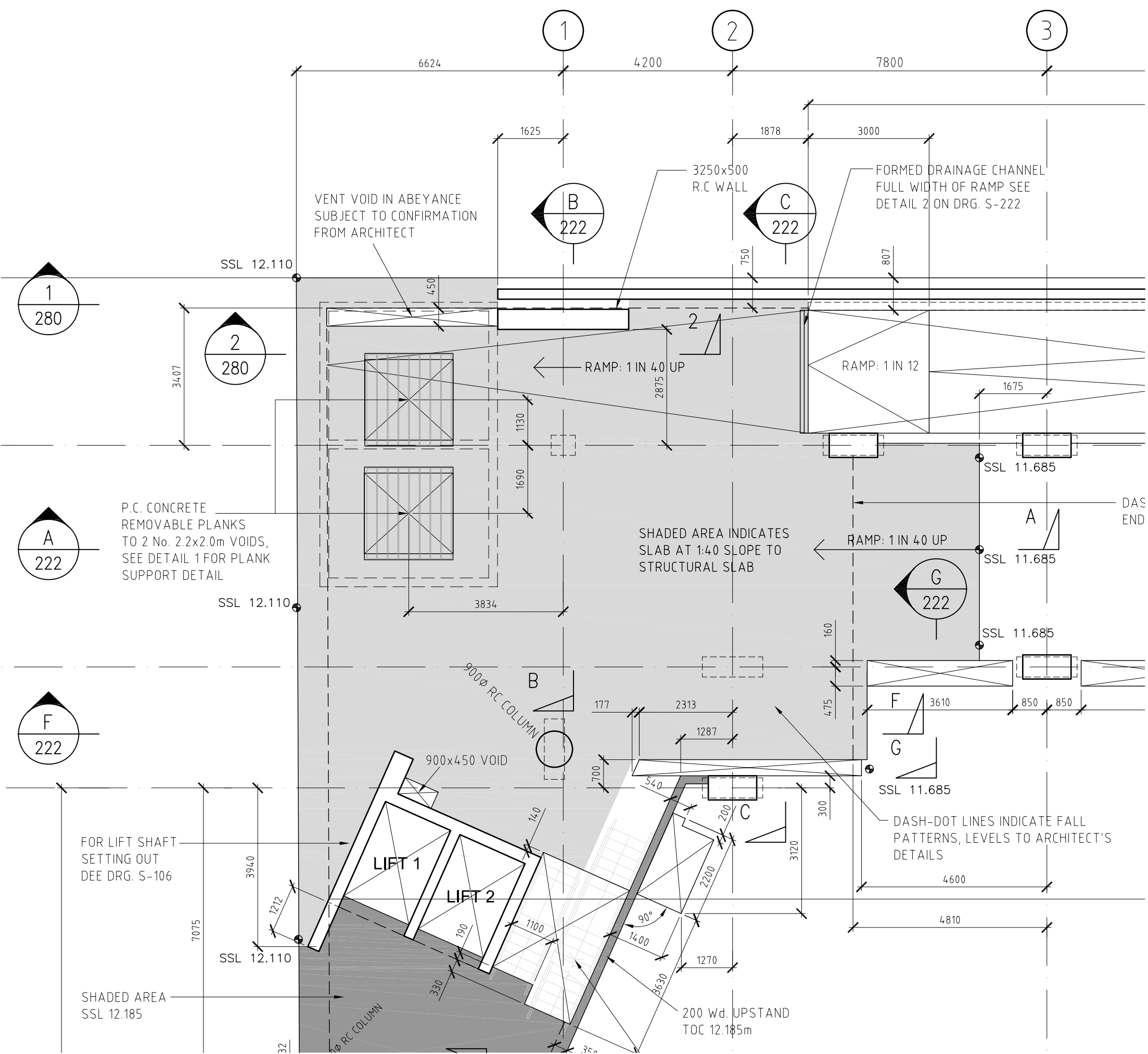
SECTION A 106/106 SECTION BETWEEN GRIDS A & B
