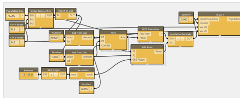
Figure 1 Implementation of NSGA-II in Dynamo to optimize daylighting and energy use
