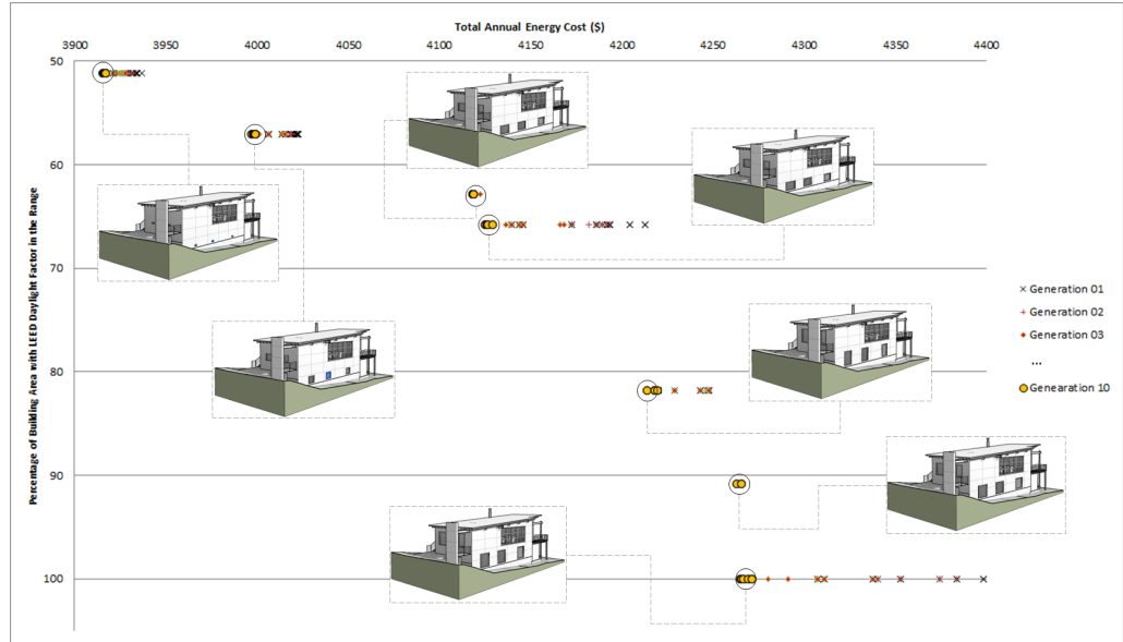
Figure 5 Scatterplot showing the Pareto Frontier with model thumbnails superimposed on the plot to illustrate the association between the calculated optimal solutions and the building forms.
