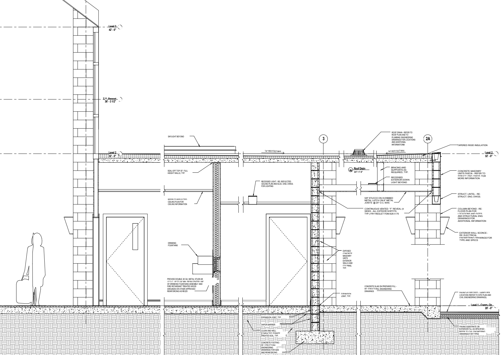
1 Section - High Corridor Wall 3/4" = 1'-0"
