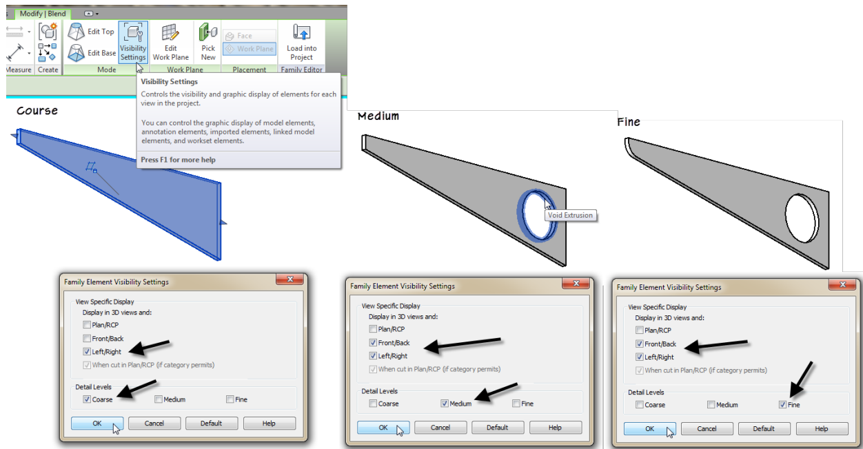
Figure 30—Course, Medium and Fine 3D geometry
