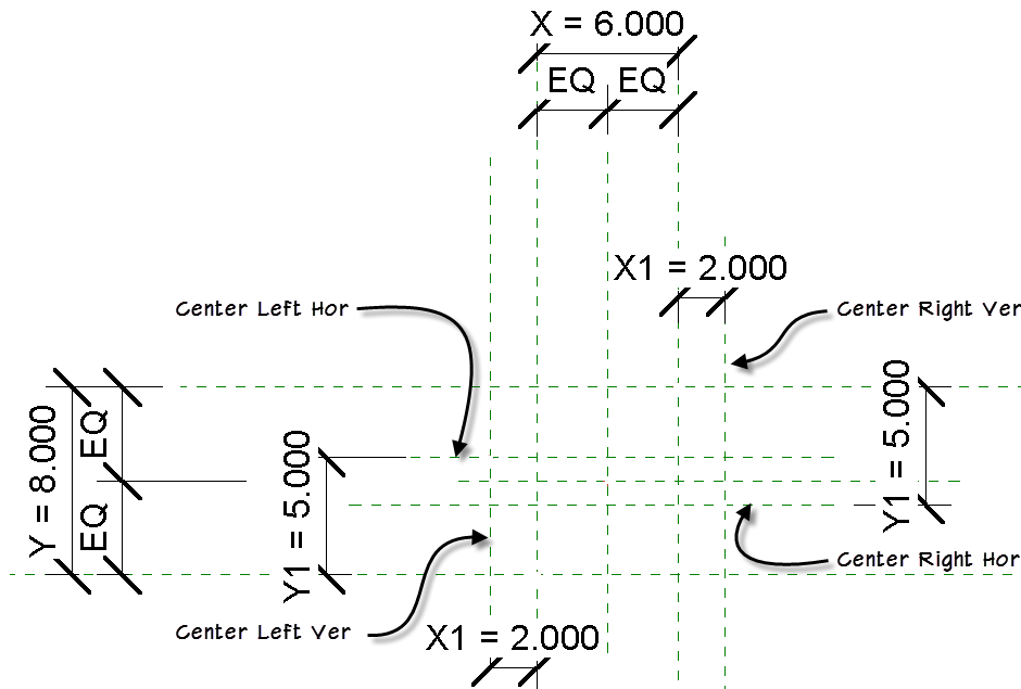
Figure 36— Create new reference planes and parameters
