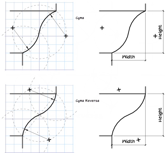
Figure 34—Constructing Cyma and Cyma Reversa profiles
