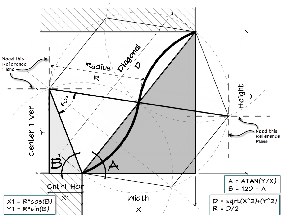
Figure 35— Applying trigonometry to locate the required Cyma reference planes
