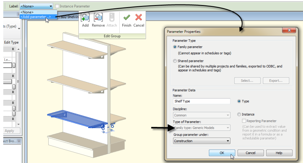
Figure 23—Create a new <Family Types> parameter
