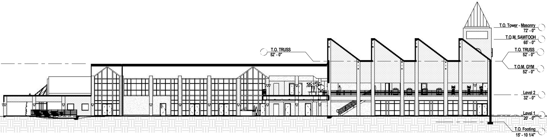
1 Section A-A Looking West 1/16" = 1'-0"
